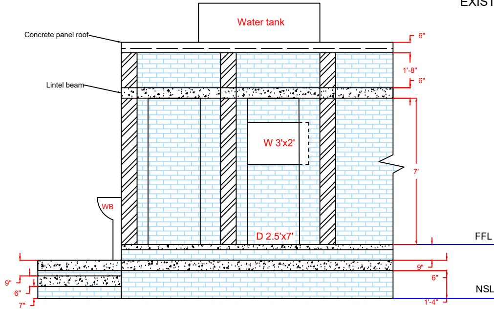
CROSS SECTION
