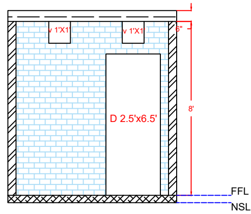
CROSS SECTION
