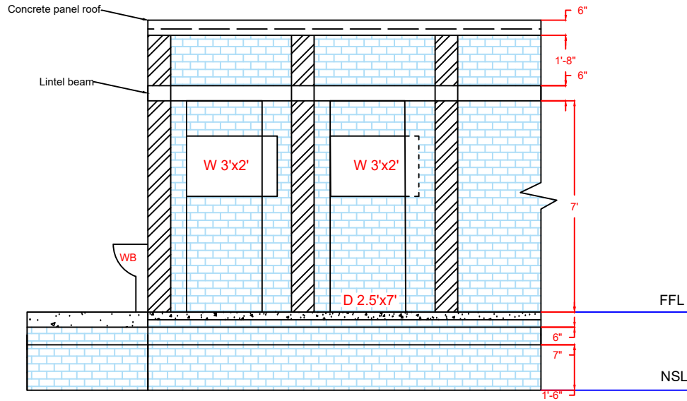
CROSS SECTION
